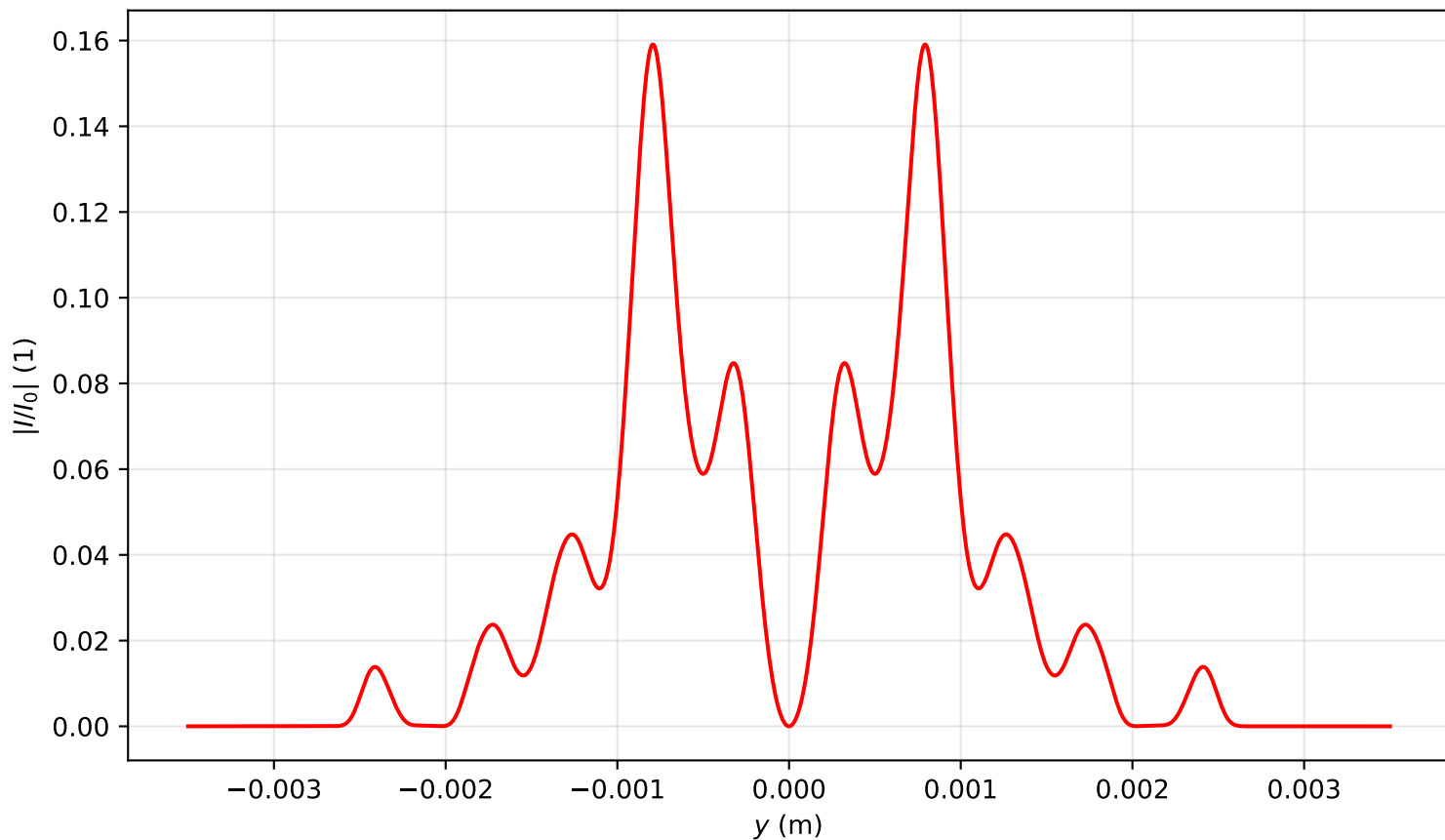
Intensity profile I(x=0, y, z=3.423)/I_0 , \text{Pin}=8.0\text{Pcr} , artificial time
